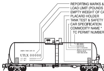
Pressure tank car Compressed liquified gases (117)
